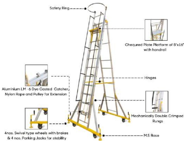
SI - 228 Alu. Telescopic Movable Ext. Ladder
