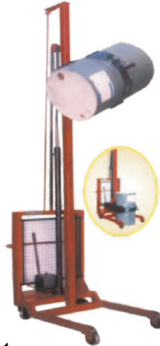
SI - 181 Drum Jockey Capacity: 350kg / 500kg Wheels: PU / Nylon / CI
