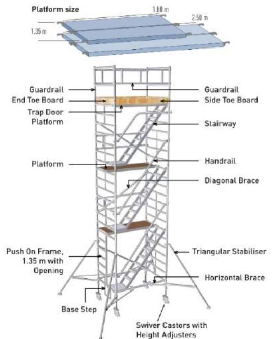
SI - 229 Alu. Scaffolding Mobile Scaffold Towers With Stairway
