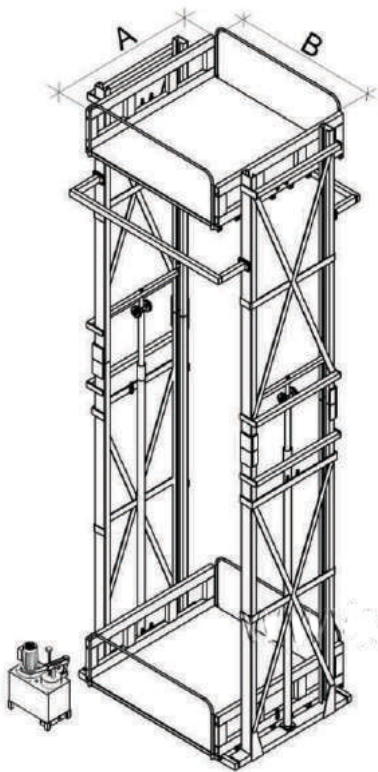
Double Mast Type
